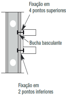
Corte vertical
