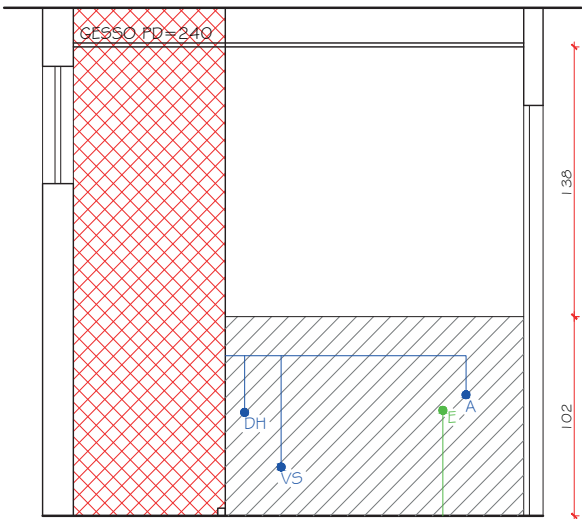
VISTA 01 - BANH SOCIAL E5C.: 1/25
